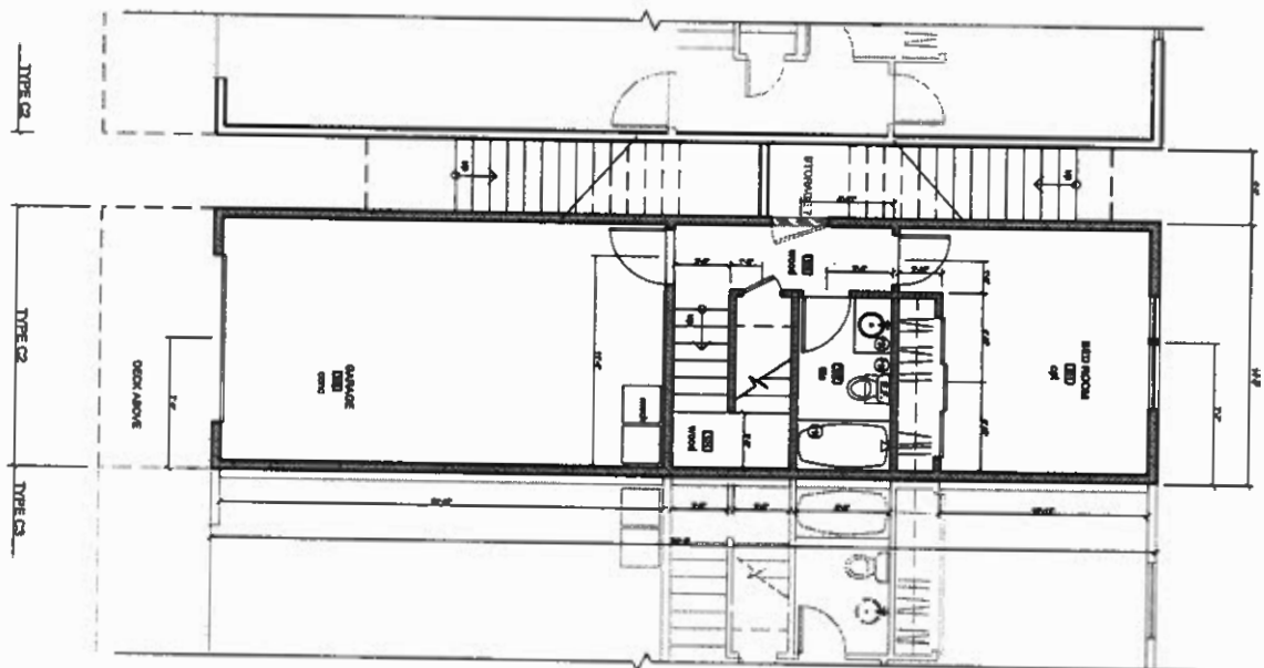
1 FIRST FLOOR PLAN
