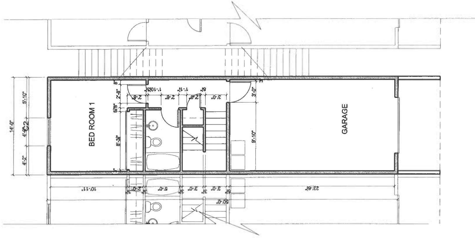
2 BEDROOM, 2 STORY, DEED RESTRICTED UNIT @ WESTERN EDGE 1 FIRST FLOOR PLAN TYPE C 2 1/8" = 1' - 0"
