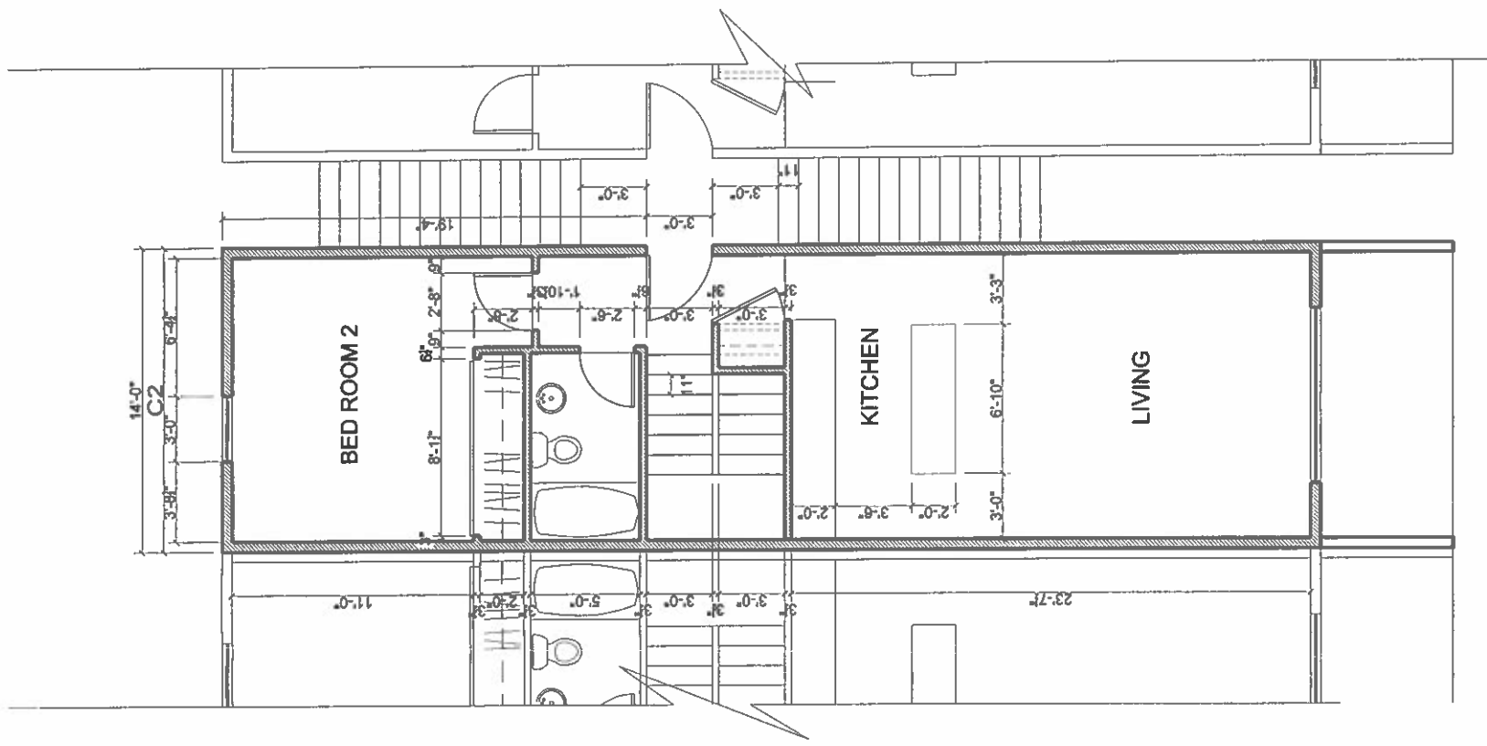
2 BEDROOM, 2 STORY, DEED RESTRICTED UNIT @ WESTERN EDGE 2 SECOND FLOOR PLAN TYPE C 2 1/8" = 1' - 0"
